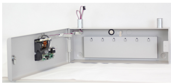
Internal View
