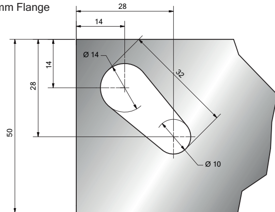
50mm Flange
