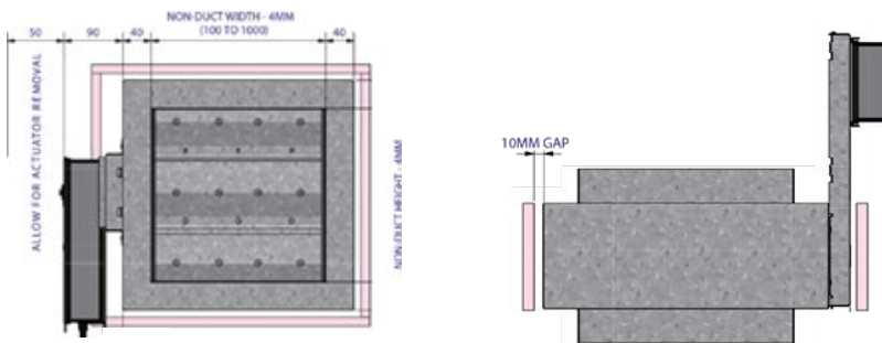
Fig. 2: FSD-TD Drywall Spacing
