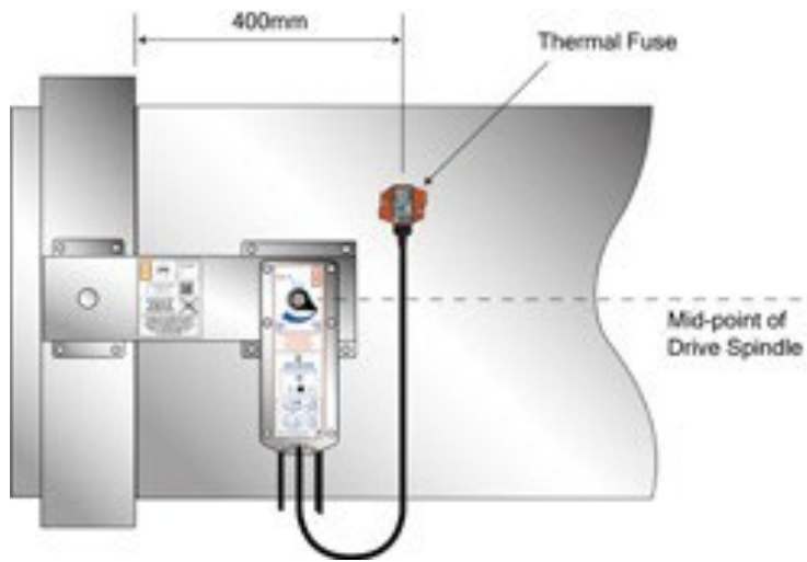
Fig. 1: Thermal Fuse (TF)
