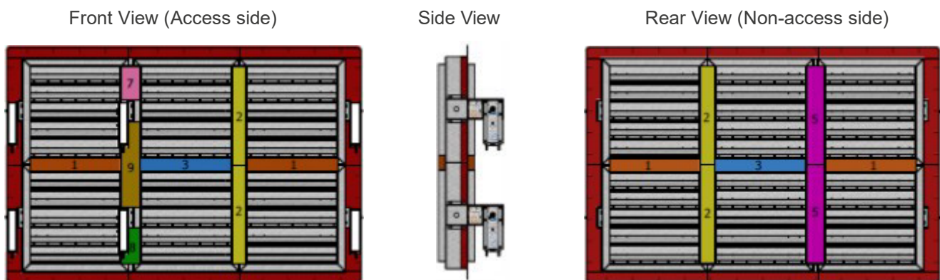
Fig. 9: Joining Channels
