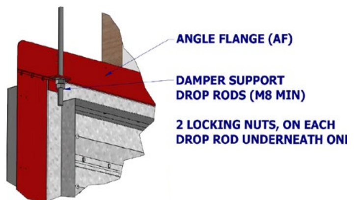
Fig. 8: Drop-rod locking nut application
