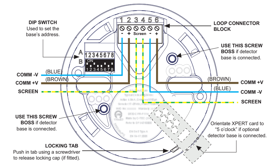
Figure 1 - Loop Connections (Typical)
