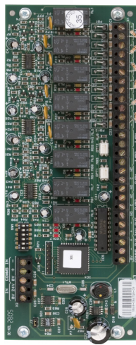
6 Way Sounder Extender Board (K546)
